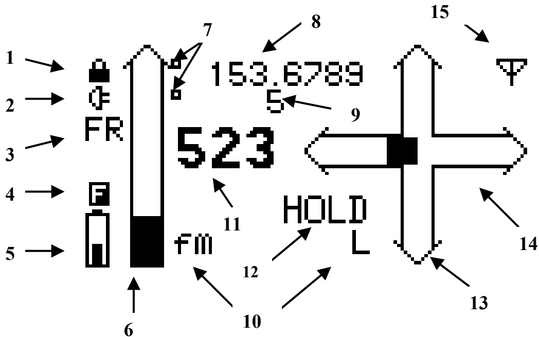
Figure 1. Display Screen Condition Indicators
